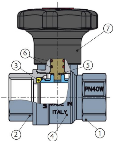
PART LIST
